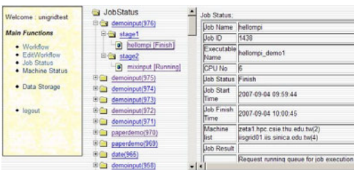
Figure 8. Job status monitoring pages
