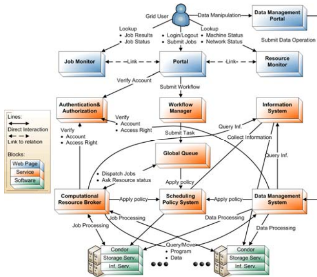
Figure 1. Component diagram for Taiwan UniGrid.
