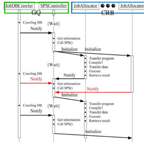
Figure 3. Sequence diagram of computing service.
