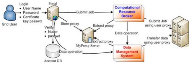
Figure 2. Single sign-on mechanism.
