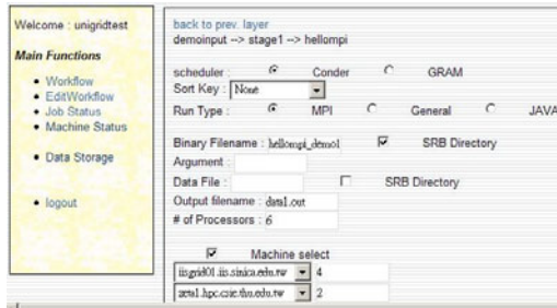
Figure 7. Job description in stage 1.
