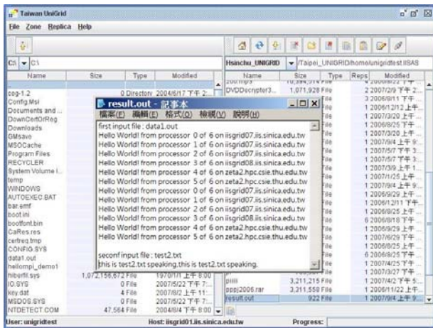
Figure 9. A screenshot of the data management client.
