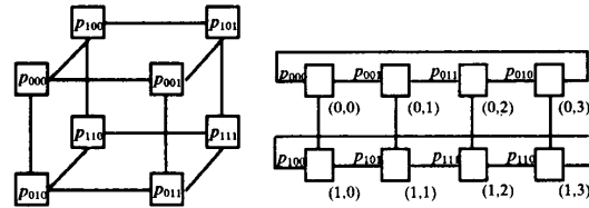
Figure 4(d): A 3-cube. Figure 4(e): Emulate a 2 \times 4 mesh.
