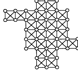
(b) The communication needed between nodes.
