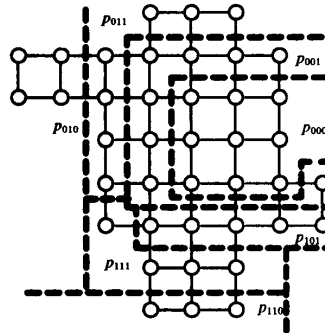
Figure 4(g): Allocate nodes to processors by using Equation 7.
