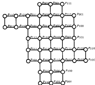
Figure 5 : Mapping a FEG onto a hypercube by using the greedy assignment mapping.
