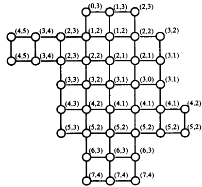
Figure 4(c): The 2-tuple labels assigned to nodes.
