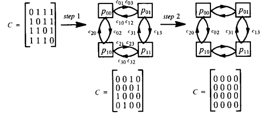
Figure 3(a) : The communication behavior of algorithm bidirectional_comm_cost .
