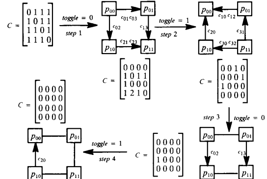
Figure 3(b) : The communication behavior of algorithm unidirectional_comm_cost .
