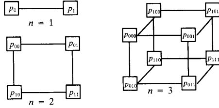
Figure 1: An example of n -cubes, for n = 1, 2 , and 3
