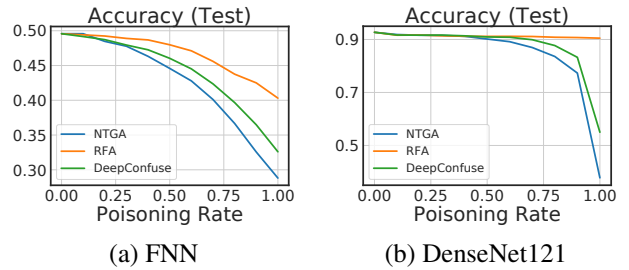
Figure 6. Partial data poisoning on CIFAR-10.
