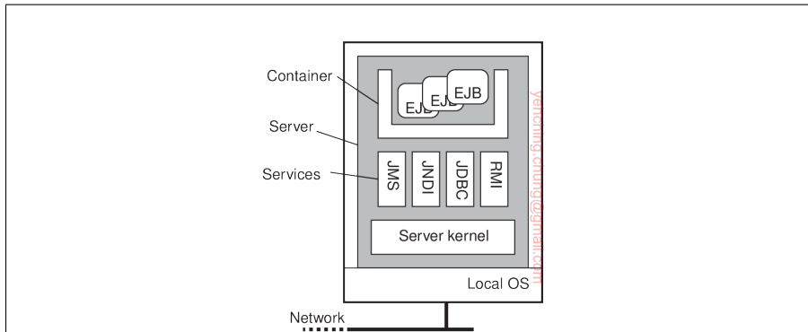
Figure 3.16: General architecture of an EJB server.
