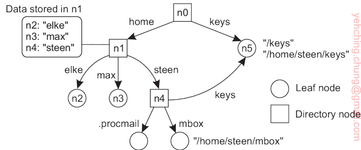
Figure 5.11: A general naming graph with a single root node.
