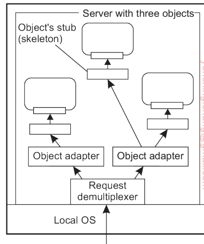
Figure 3.14: An object server supporting different activation policies.
