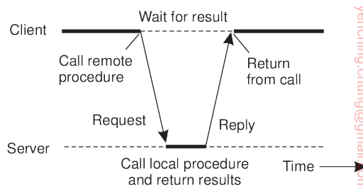
Figure 4.6: The principle of RPC between a client and server program.
