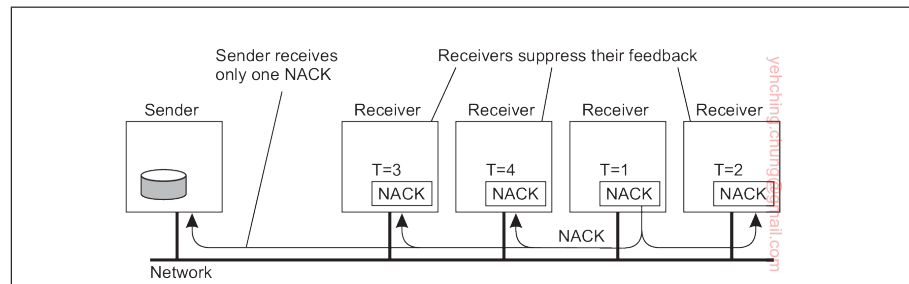
Figure 8.23: Several receivers have scheduled a request for retransmission, but the first retransmission request leads to the suppression of others.
