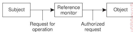
Figure 9.19: General model of controlling access to objects.
