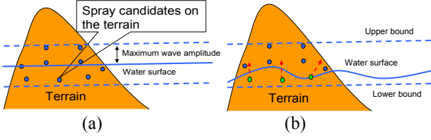
Fig. 3. (a) The blue particles are those candidates to simulate spray. (b) The green particles are set to active due to their positions are under water and emitted along the predefined directions.
