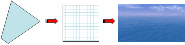
Fig. 1. The left is the visible ocean region in object space. The middle is the corresponding screen-space rectangle discretized to a regular grid which is represented as a vertex texture. The right is the corresponding region with applying waves on it.
