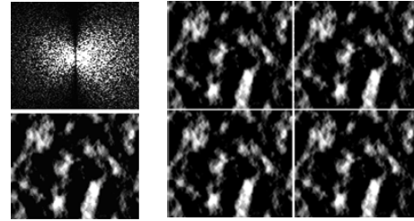
Fig. 2. The left are the random Fourier amplitudes of ocean waves and the corresponding height map. The right is a height map spanning over an unbounded water surface.
